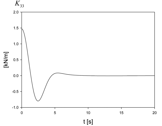
Fig. 5. Impulse response function for heaving buoy.
